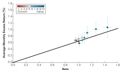
Excess Return of Book-to-Market Portfolios, 1926-2015
